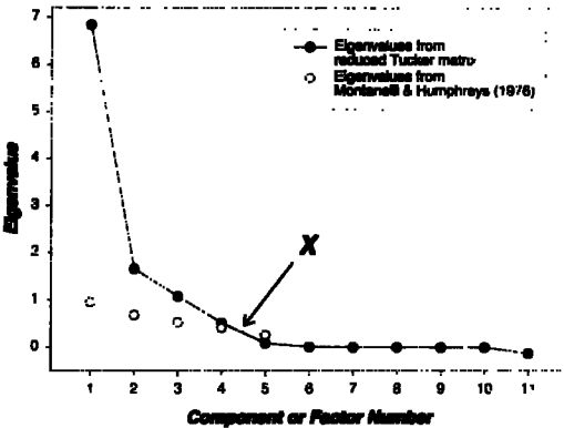
FIGURE 3 Superimposed scree plots for eigenvalues of random and real data sets including 11 measured variables, N=63 . There are four eigenvalues before the last big drop, indicating that four factors should be retained. It is evident by using parallel analysis that four factors should be retained.
