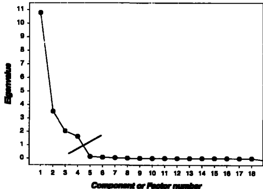
FIGURE 1 A scree plot for a correlation matrix of 19 measured variables. The data were obtained from a version of the Tucker matrix (discussed later) with additional variables. There are four eigenvalues before the last big drop, indicating that four factors should be retained.
